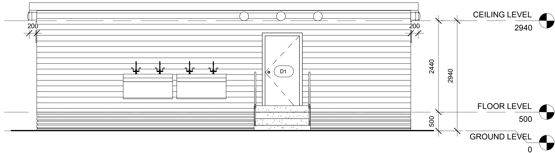
1 FRONT ELEVATION
