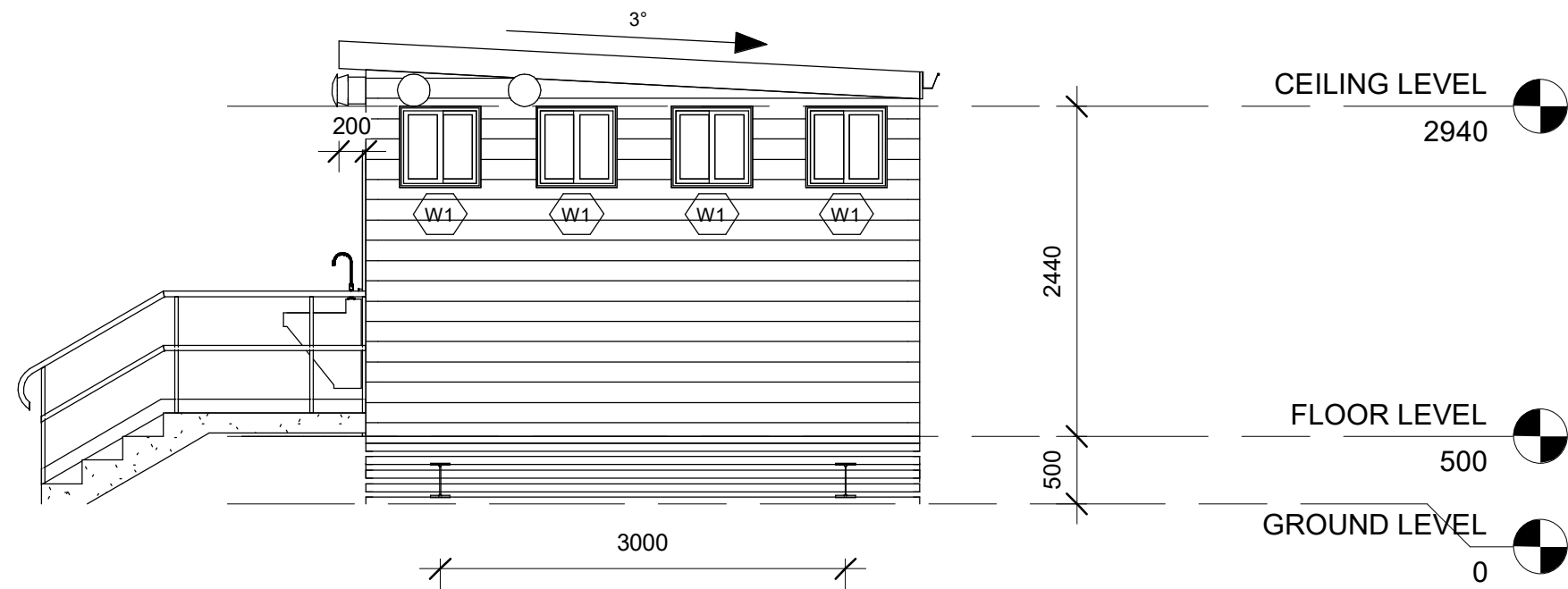
1 SIDE ELEVATION
