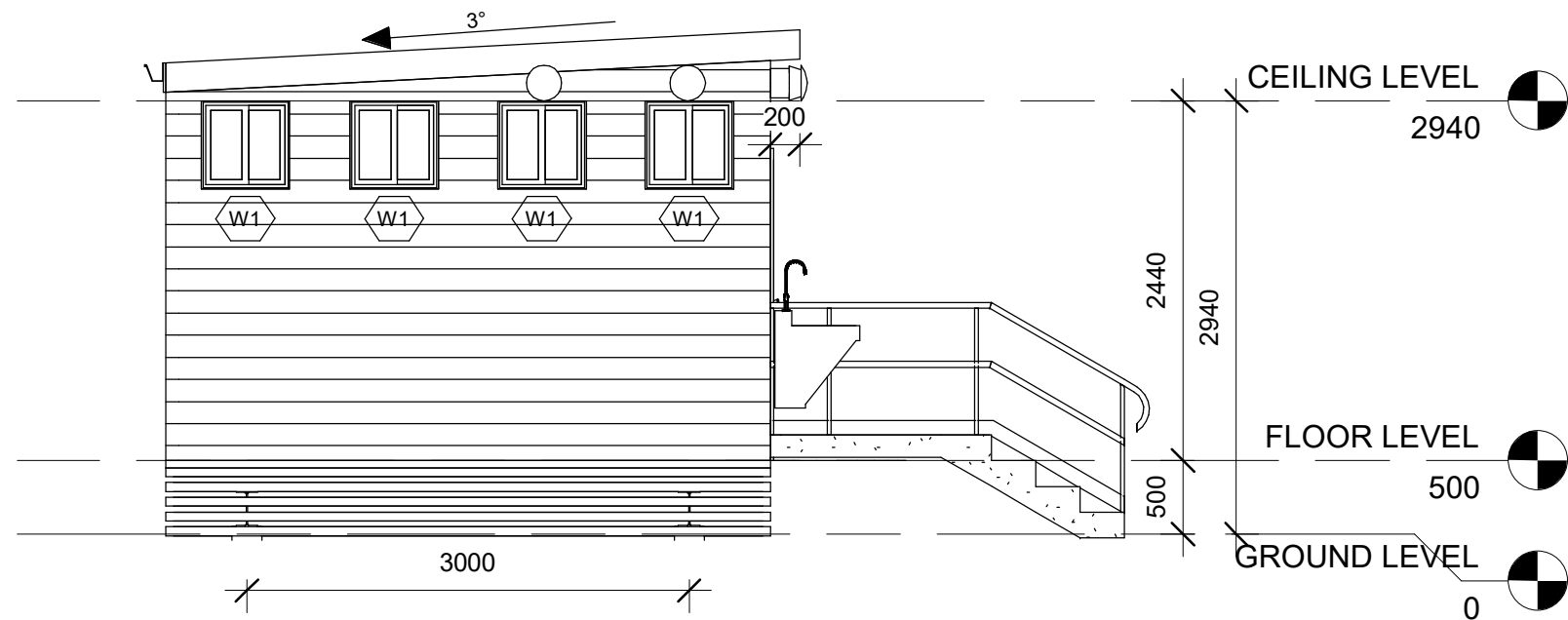
2 SIDE ELEVATION
