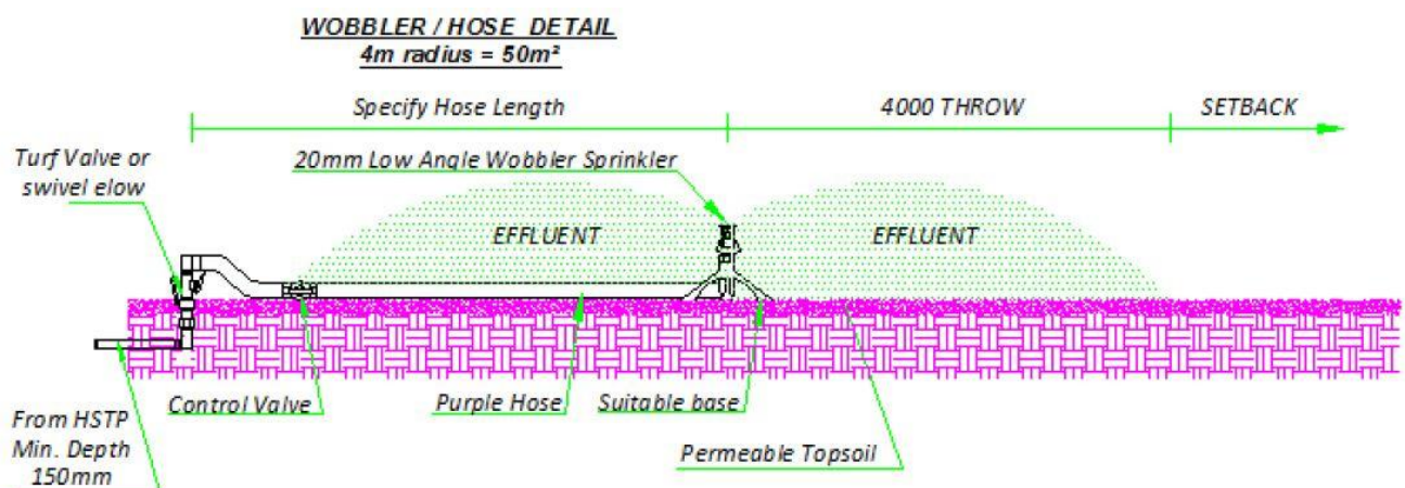
Typical Spray Irrigation Diagram
