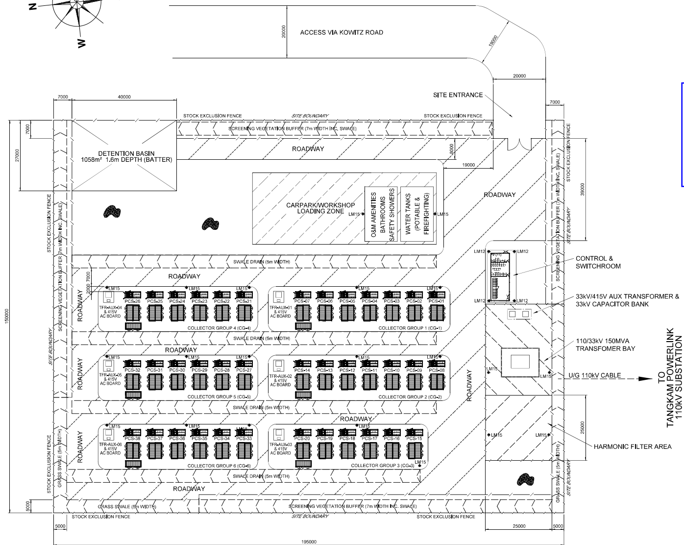
GENERAL ARRANGEMENT SCALE: 1:500
