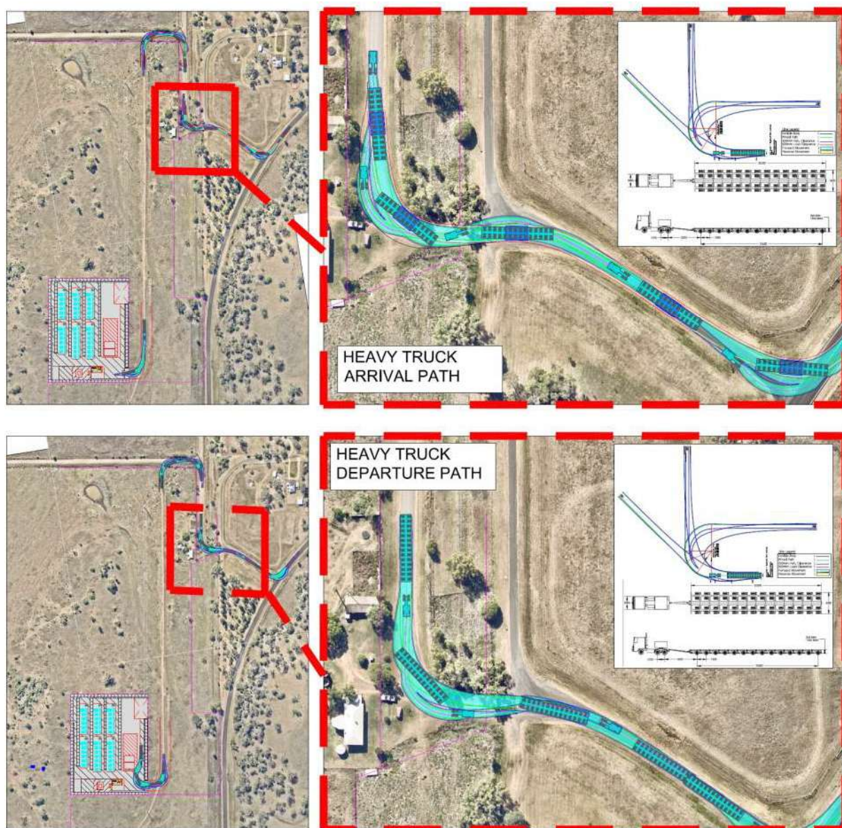
FIGURE 4.6 – SWEEP PATH OF OVERSIZE VEHICLE AT THE KEARNEY ROAD / BRENNAN ROAD INTERSECTION
