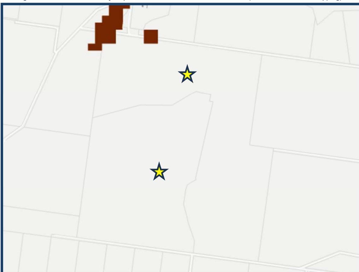
Figure 8: Landslide Hazard Overlay map of sites and surrounds
