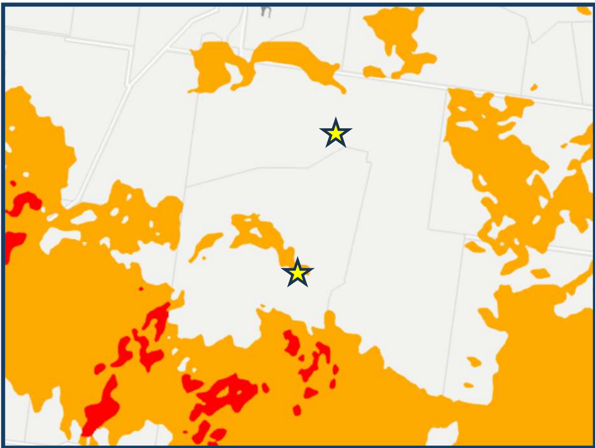
Figure 5: Bushfire Hazard Overlay map of sites and surrounds
