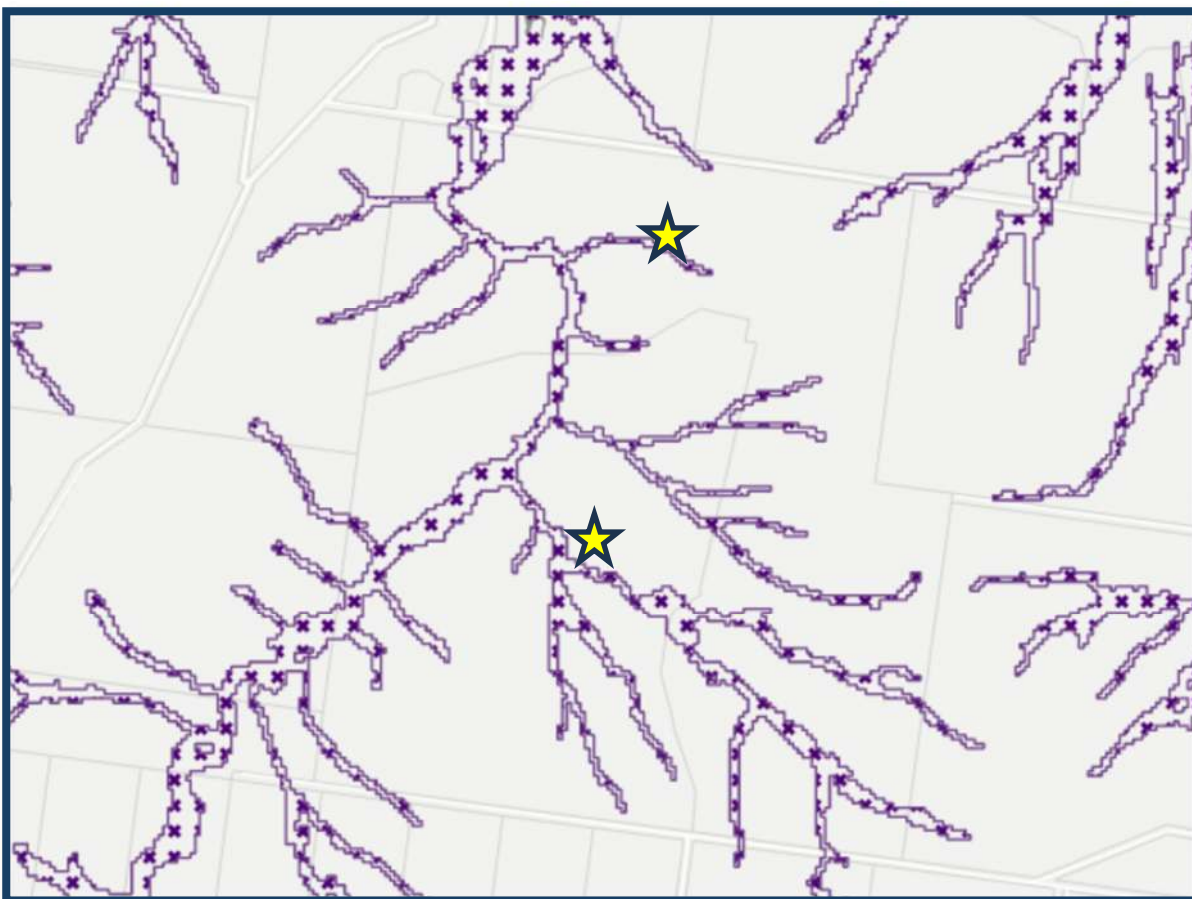
Figure 7: Flood Hazard Overlay map of sites and surrounds
