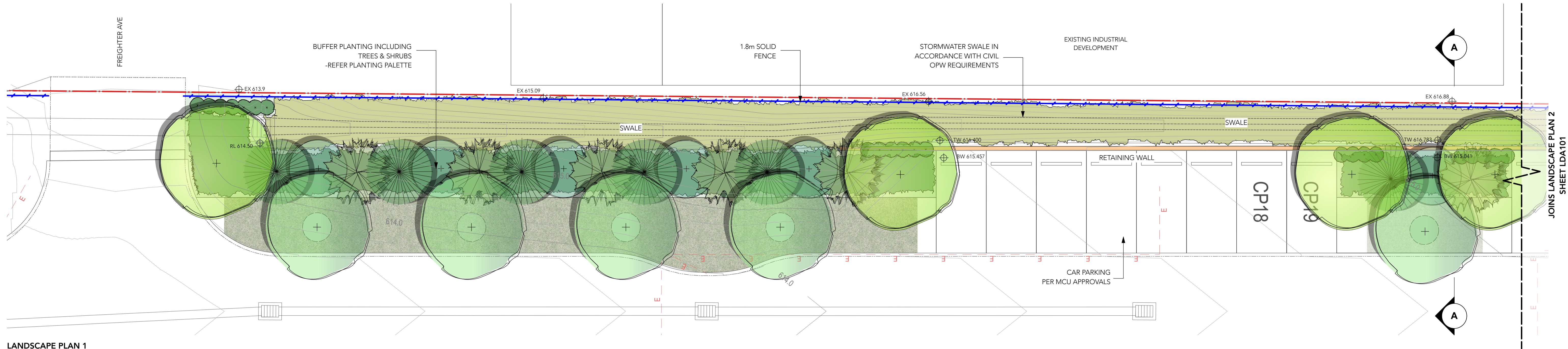
LANDSCAPE PLAN 1 SCALE: 1:100 @A1
