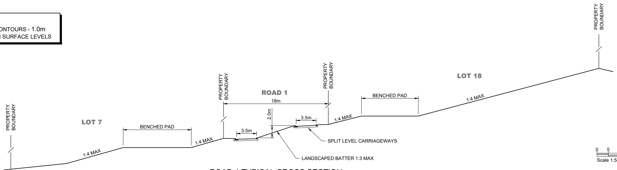
ROAD 1 TYPICAL CROSS SECTION NTS
