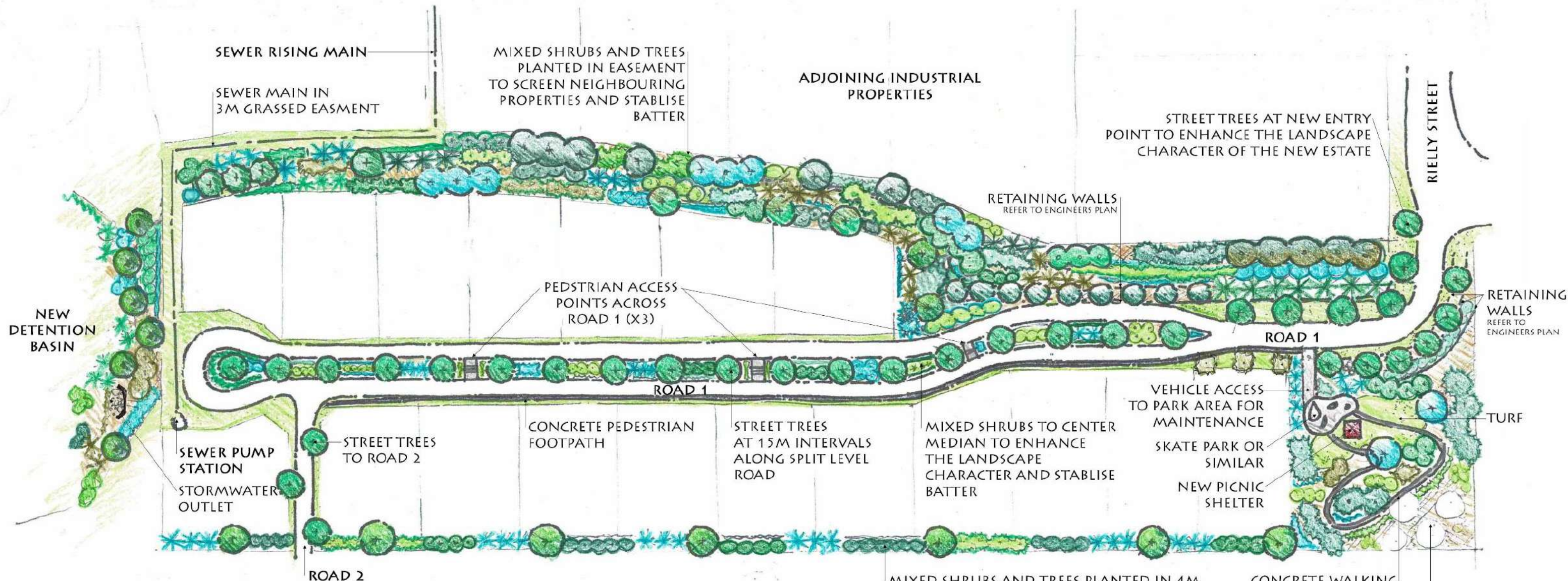
CONCEPTUAL LANDSCAPE PLAN SCALE 1:1000
