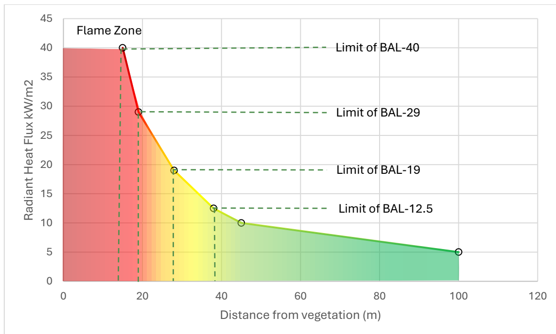
Figure 18 Potential radiant heat flux versus distance from bushland areas (VHC 12.1)
